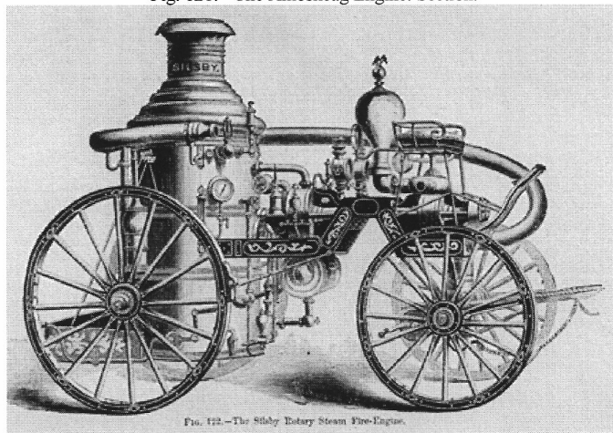
Fig. 122. - The Silsby Rotary Steam Fire-Engine.
