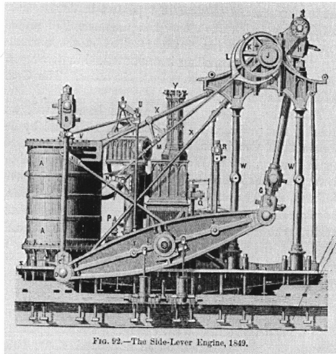
Fig. 92. - The Side-Lever Engine, 1849.
