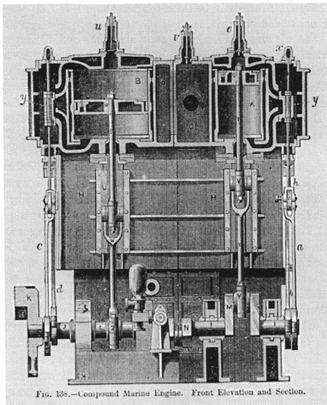
Fig. 138-Compound Marine Engine. Front Elevation and Section.
