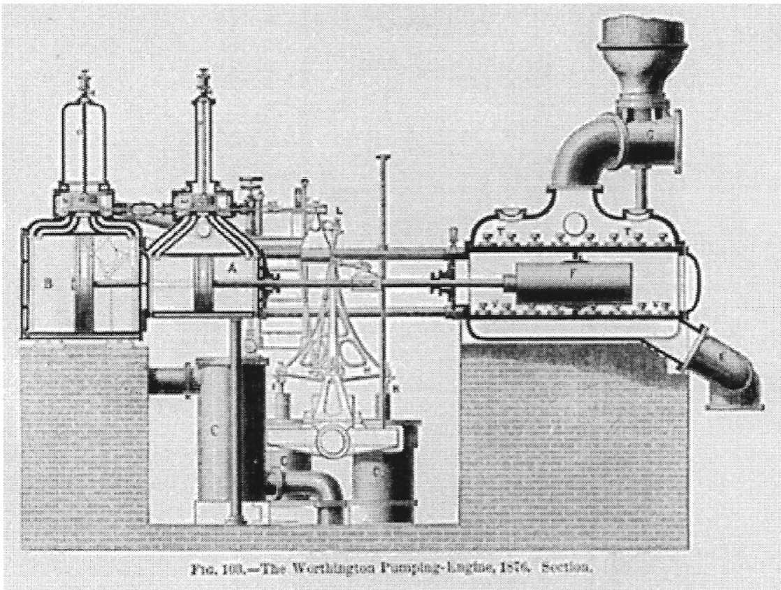
Fig. 103.-The Worthington Pumping-Engine, 1876. Section.
