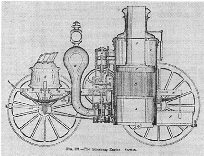
Fig. 121. - The Amoskeag Engine. Section.
